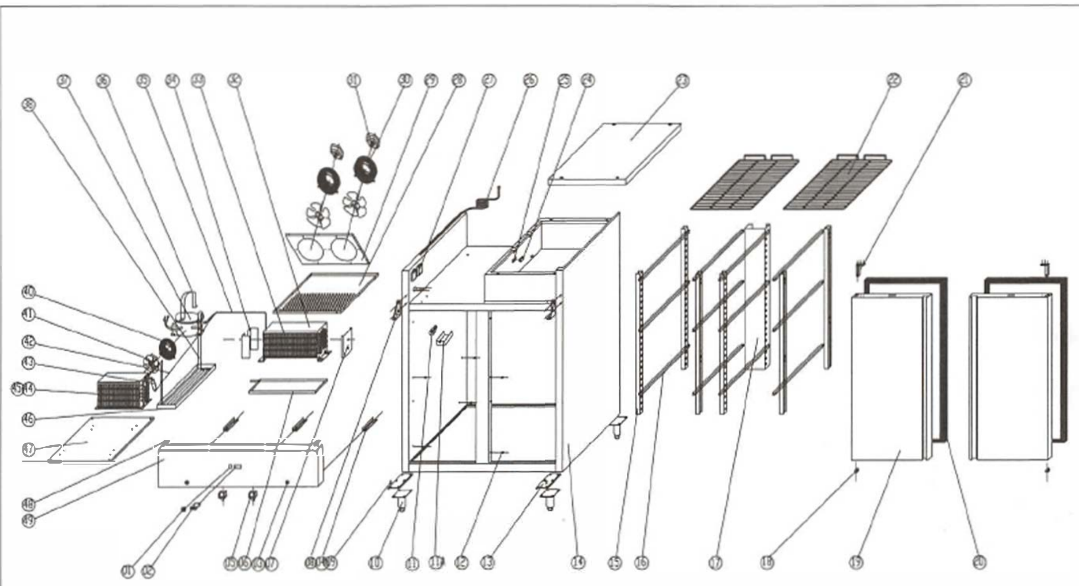
EXPLODE DIAGRAM OF RNG1410TN
